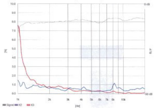
LCY Ribbon (2.83V / 0.25M)
