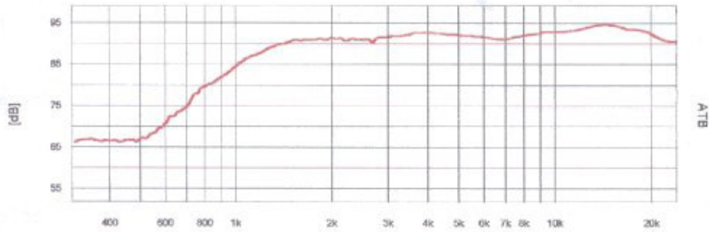
LCY-130 Ribbon (2.83V / 1M)
